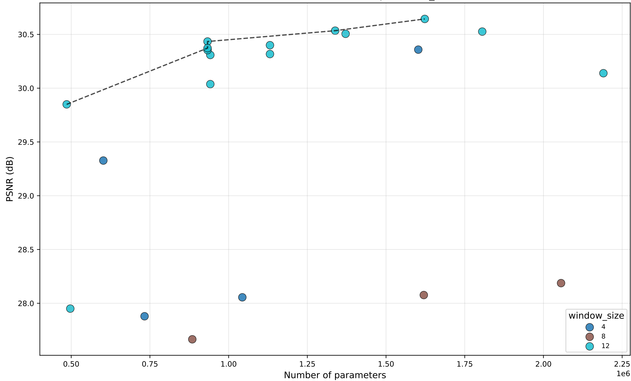
PSNR vs #Params — ELAN — by window_size
